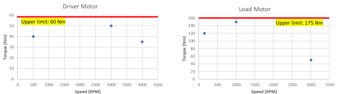
Figure 2: Critical points on the torque-speed graph of motors
