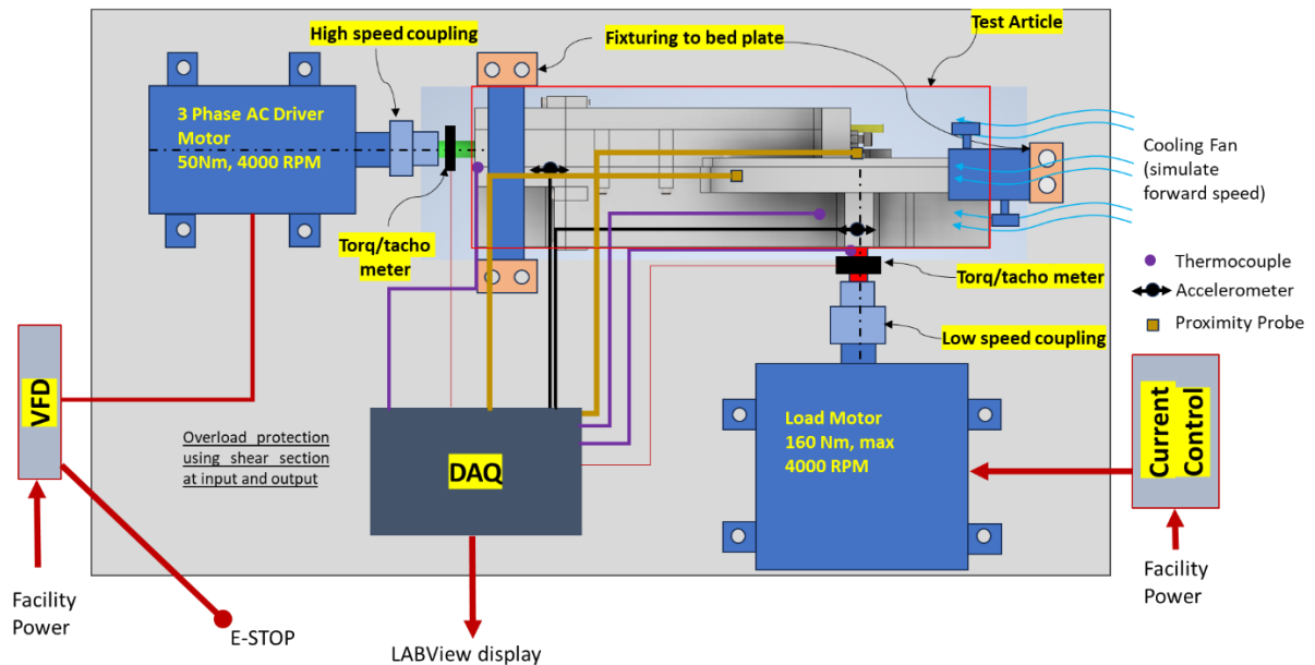
Figure 1: Test rig for traction drive prototype
